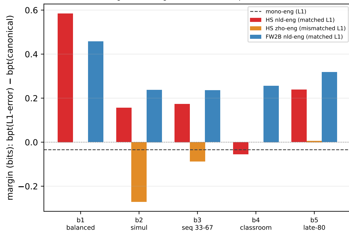
(C) BLISS — every Beetle model >chance on learner-error preference (D) §4.2 L1-transfer simulation — matched bilingual disambiguates; mismatched produces the canonical L1-transfer error (negative margin)
