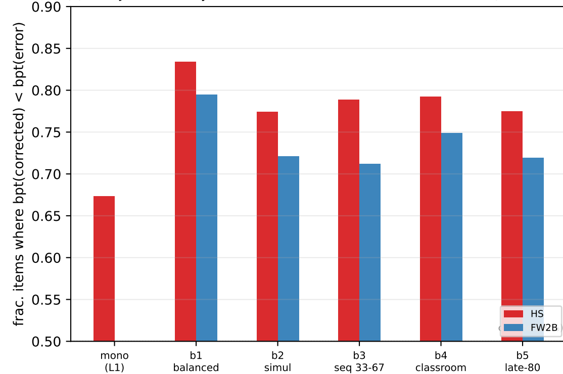
(F) §4.2 JFLEG — every Beetle model ranks corrected > learner-error (frac > 50%)
