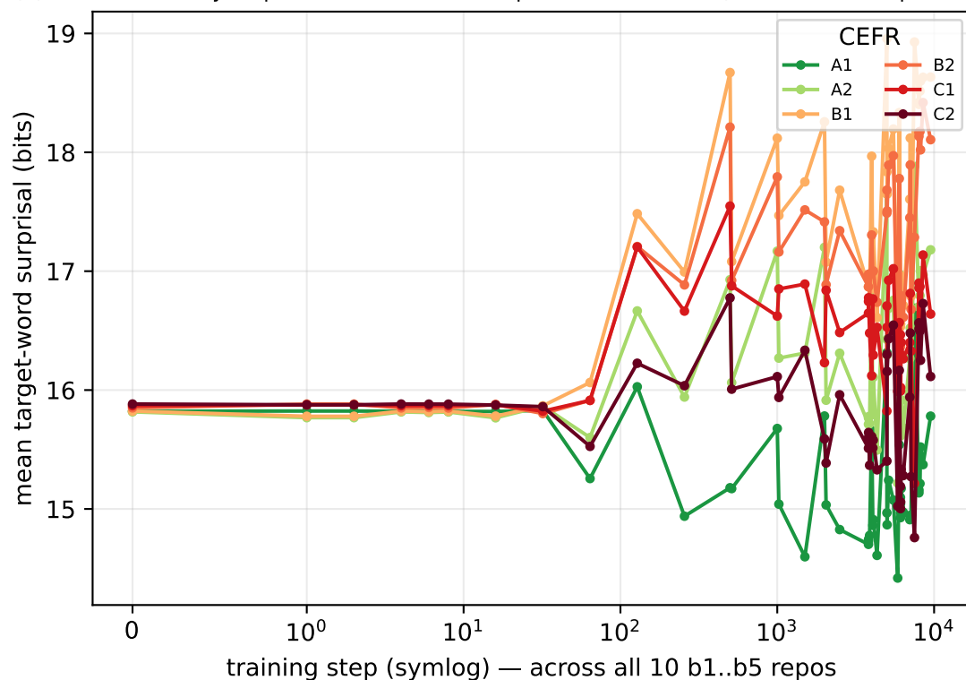
(E) §4.3 Vocabulary acquisition — A1 words drop first, then A2..C2 (canonical L2 acquisition order)
